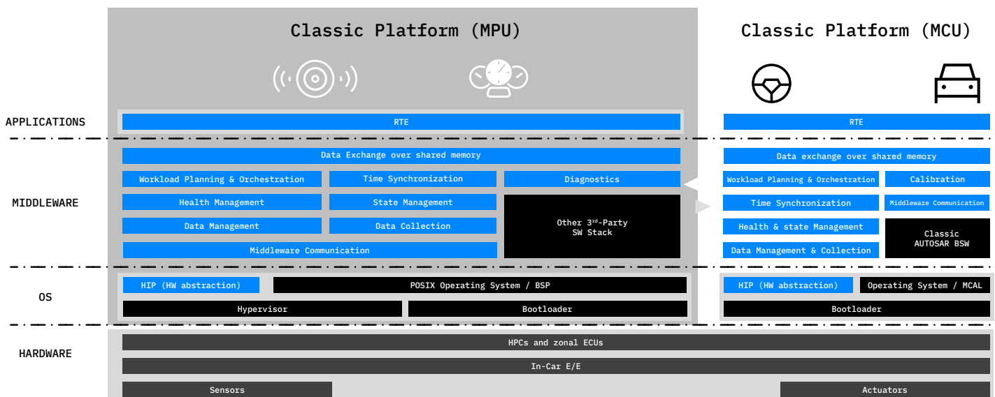
Figure 2 Layered Block diagram of the reference MotionWise Classic Platform
